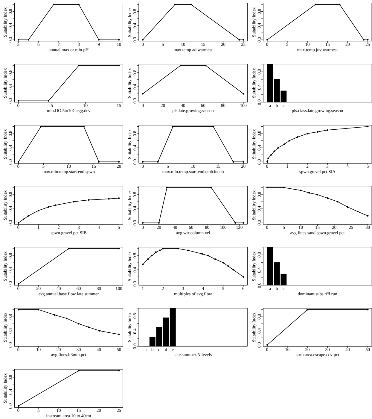
Figure 1. Suitability index graphs for variables included in the chinooksalmonLimit5to10CSand model in ecorest.
